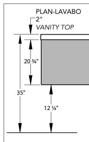
PLAN-LAVABO 2" VANITY TOP
