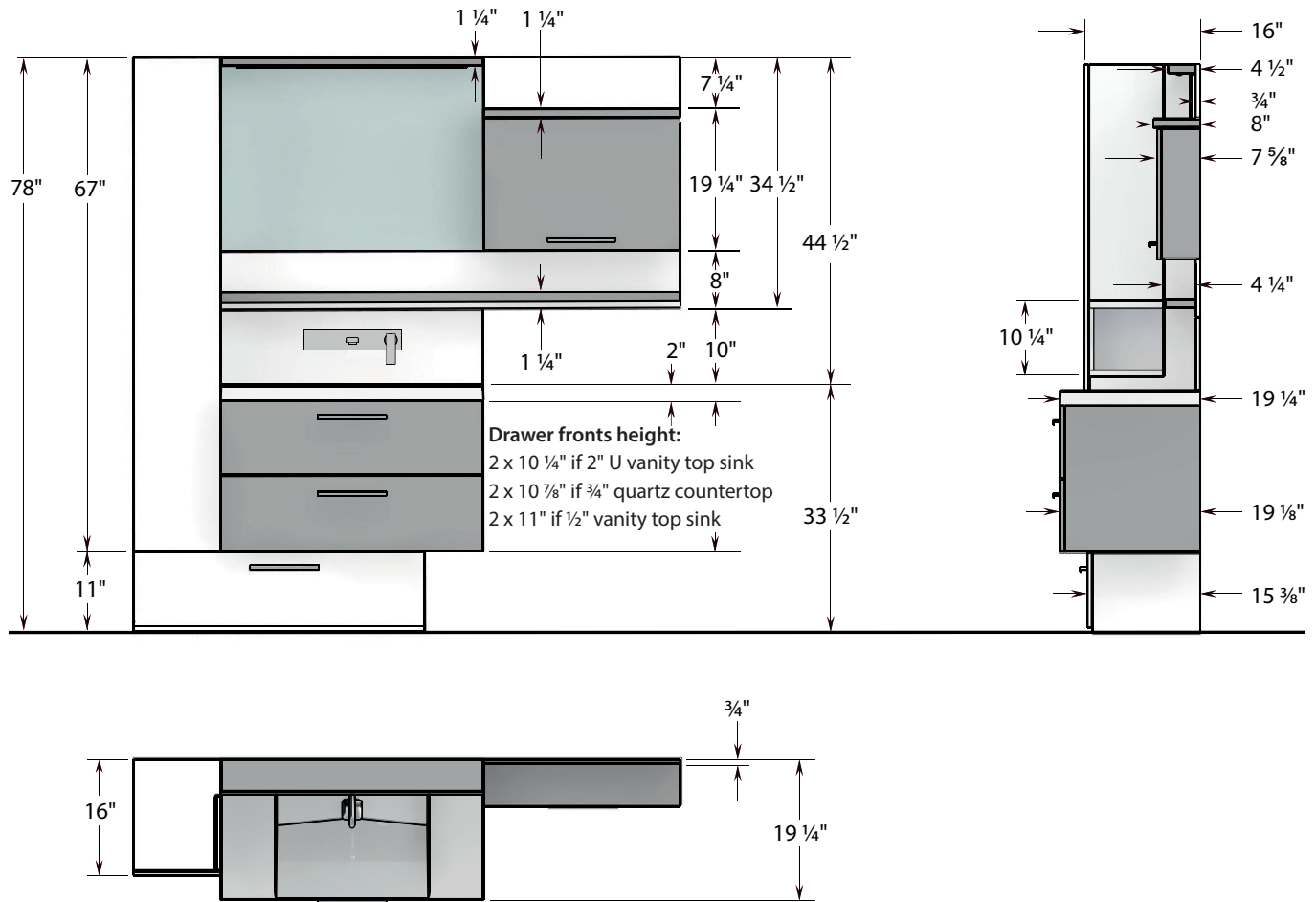
LAYOUT WITH LINEN-MEDICINE CABINET, TOE-KICK DRAWER AND EXTENDED MEDICINE CABINET
