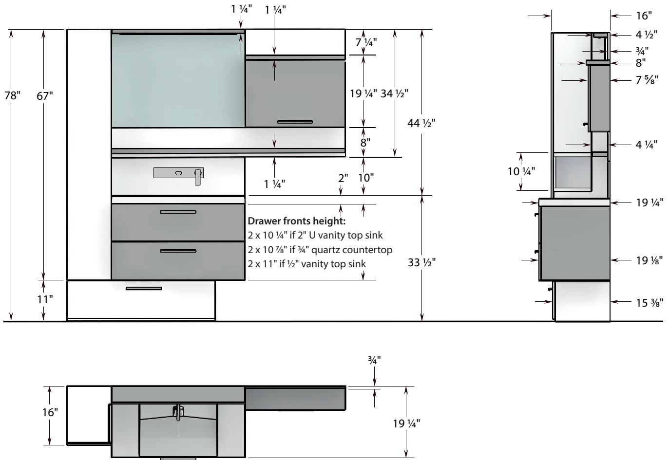
LAYOUT WITH LINEN-MEDICINE CABINET, TOE-KICK DRAWER AND EXTENDED MEDICINE CABINET
