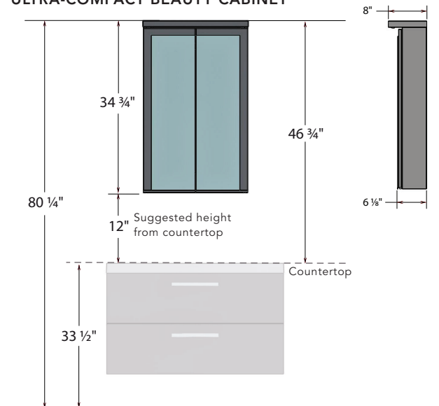
ULTRA-COMPACT BEAUTY CABINET
