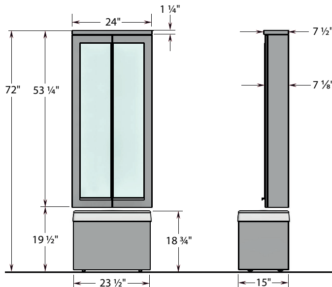
COMPACT DRESSING TABLE
