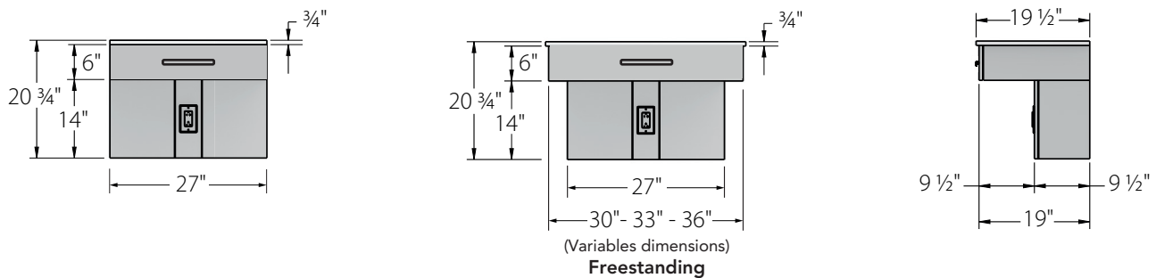
DRESSING TABLE LOWER SECTION
