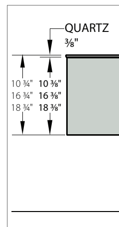
THINNED QUARTZ 3/8"
