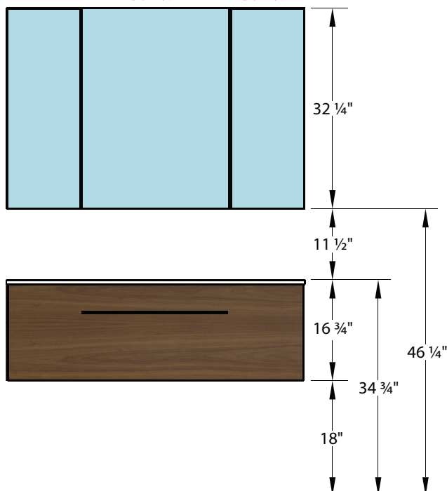
MIRROR D: 2 1/8" MEDICINE CABINET D: 4 3/8"
