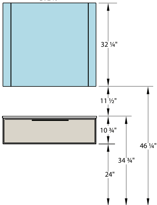
MIRROR D: 2 1/8"
