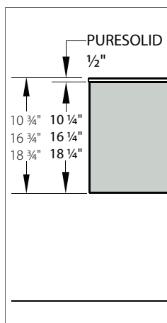
PURESOLID 1/2"
