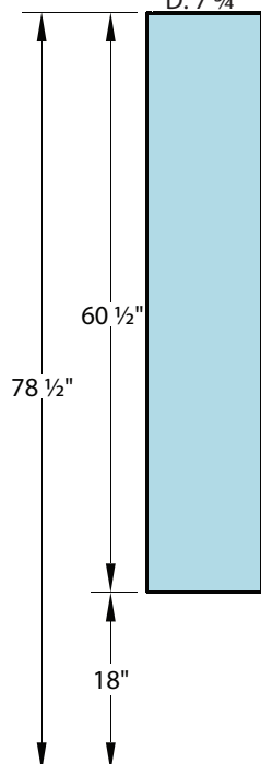
SKYLINE-16 FULL HEIGHT MED. CAB. D: 7 3/4"
